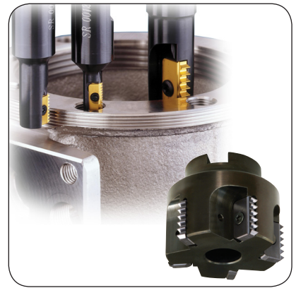
Mill-Thread
