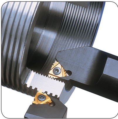
Thread Turning
